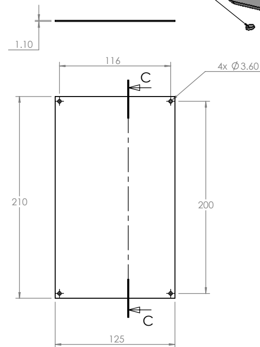
SECTION C-C
