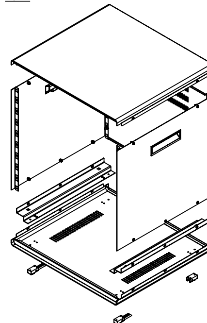
ISO VIEW 1:12
